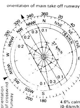
5 Typical wind rose
